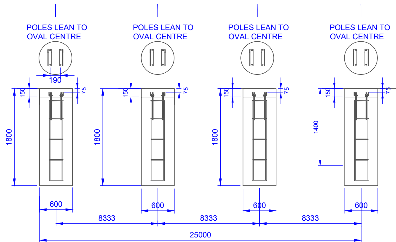
AFL GOAL NET POST FOOTING DETAILS
