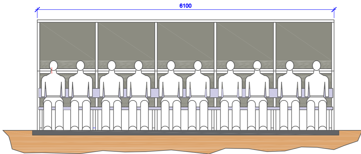
CONCRETE SLAB 6250 X 1225 X 100 MM
