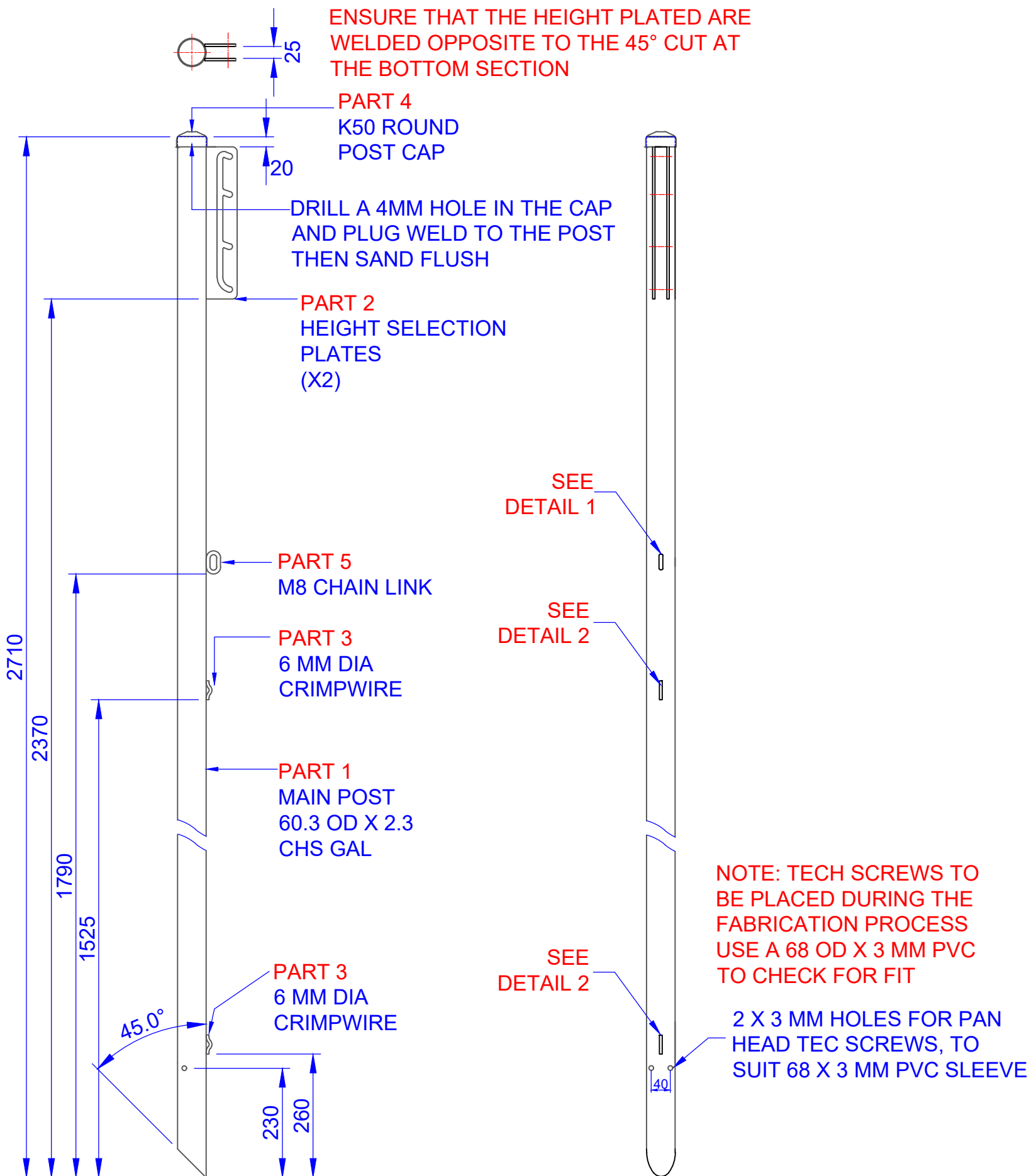
SUB ASSY 01 V60 VOLLEYBALL / BADMINTON POST QTY - 2
